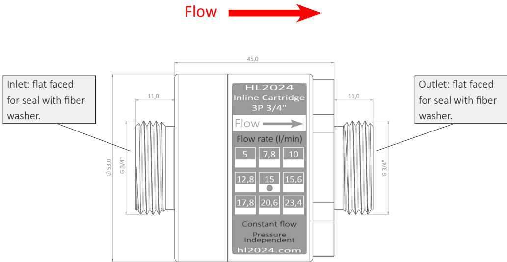
Image: HL2024 Inline Cartridge 3P 3/4" (dimensions in mm)
