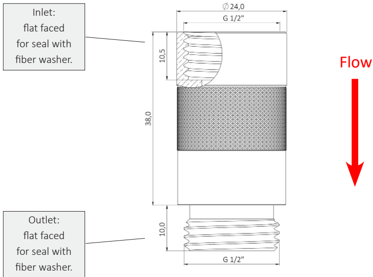
Image: HL2024 Shower (dimensions in mm)
