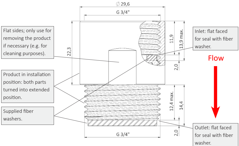
Image: HL2024 Connect (dimensions in mm)
